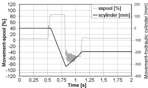
Figure 5.b Movement of the spool and the piston rod of the cylinder without any mass during the loading cycle in the water PCH
